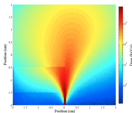
(b) Analog Benchmark
