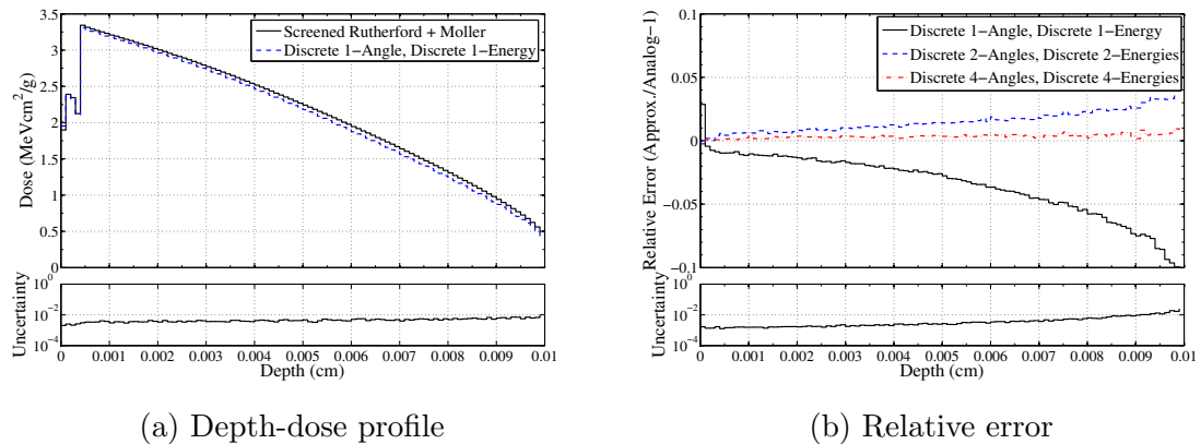
Figure 9.20: Comparison of depth-dose profiles (a) from 150-keV electrons on a gold-aluminum slab with discrete elastic scattering and discrete inelastic models. The relative error in dose (b) from 150-keV electrons on a gold-aluminum slab calculated using discrete and hybrid elastic scattering models and discrete inelastic models. The relative error is measured with respect to the numerical benchmark generated using the partial-wave expansion elastic DCS and the Möller inelastic scattering models. The associated statistical uncertainty is included below each plot.
