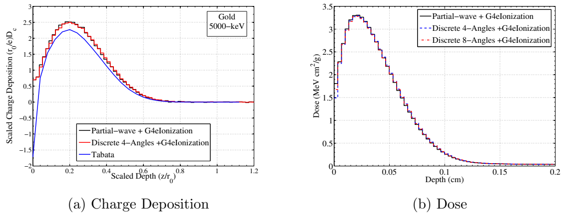
Figure 9.40: Comparison with Tabata data for 5000-keV electrons normally incident on a gold slab.
