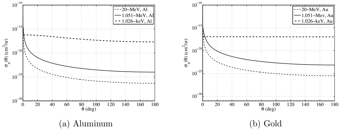
Figure 3.3: Screened Rutherford (SR) DCS for elastic scattering of 1.026-keV, 1.051-MeV, and 20-MeV electrons by aluminum and gold nuclei.
