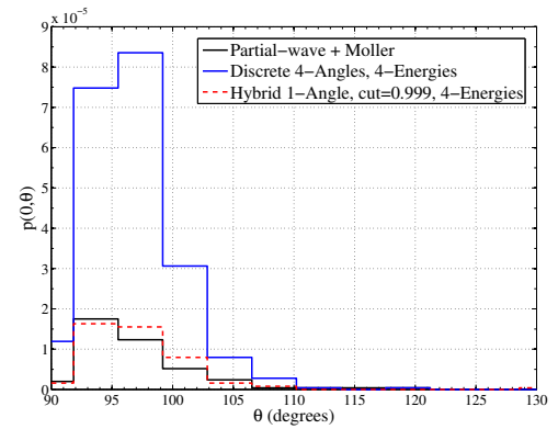
(b) 300 mfp
