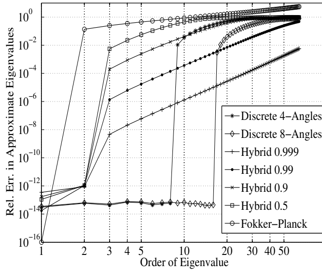
Figure 7.4: Comparison of eigenvalues of various approximations of the elastic collision operator for 1-MeV electrons colliding with gold.
