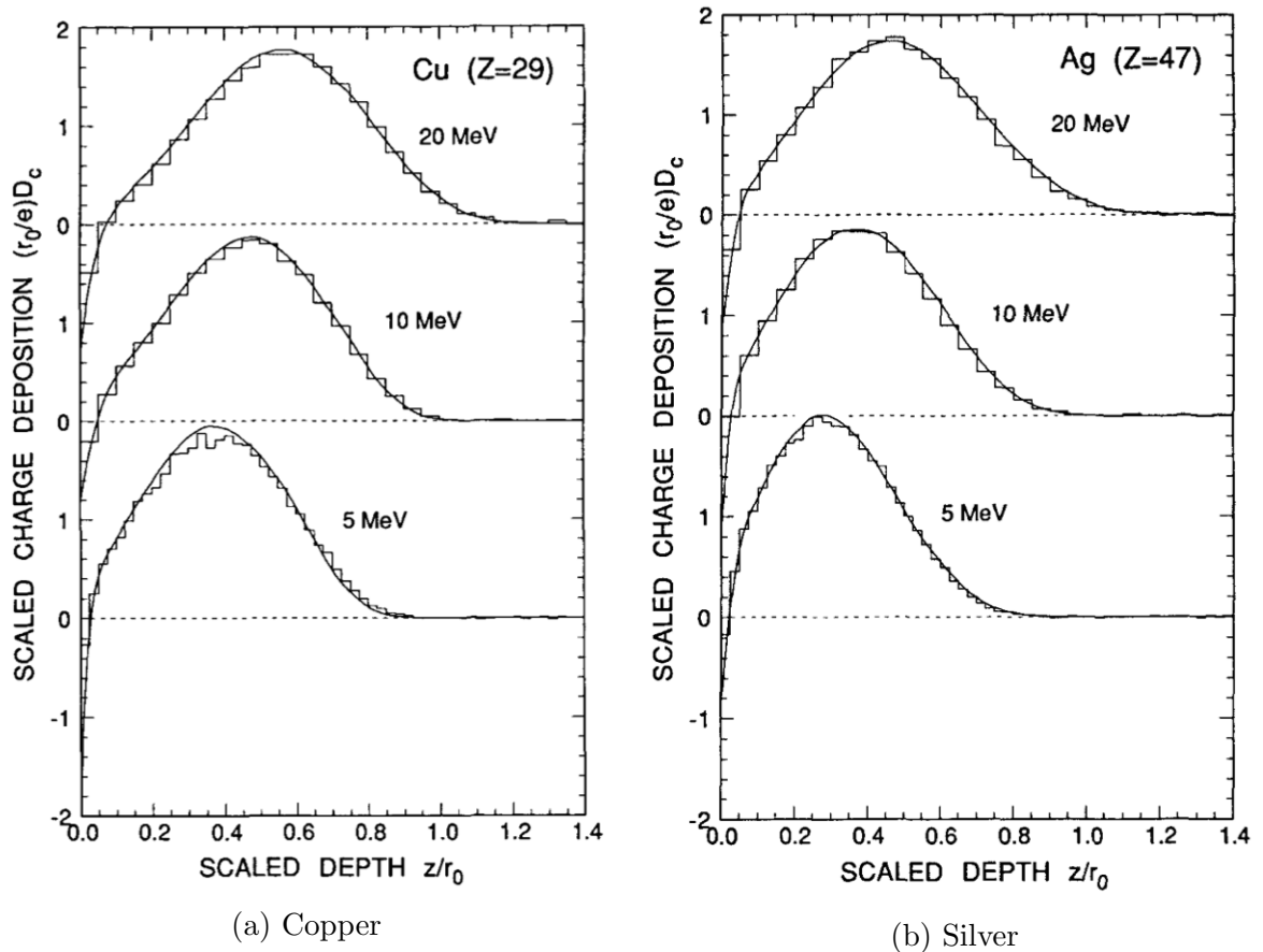
Figure 10.5: Charge-deposition distributions by 5, 10, and 20 MeV electrons incident on copper and silver. Histograms, ITS Monte Carlo results; curves, experimental results obtained by the interpolation of data.
