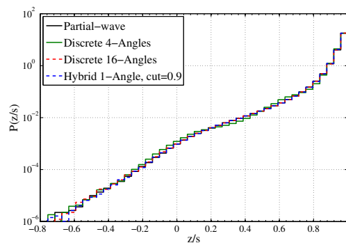
(b) 300 mfp
